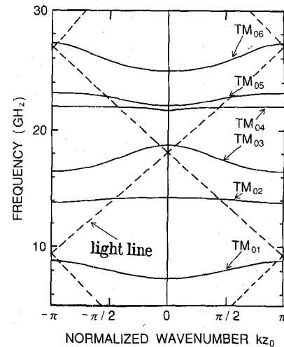
Fig. 2. Numerically obtained dispersion relations of the SWS for -\pi \leq k z_0 \leq \pi in the first Brillouin zone. The parameters of the SWS are: R_0 = 1.4499 cm, z_0 = 1.67 cm, and h = 0.406 cm. Light lines ( \omega/k = c ) are shown by dashed lines.
